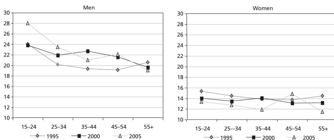
Figure 17 Trends in the generic physical risk factor, by age and sex, EU15, 1995–2005
